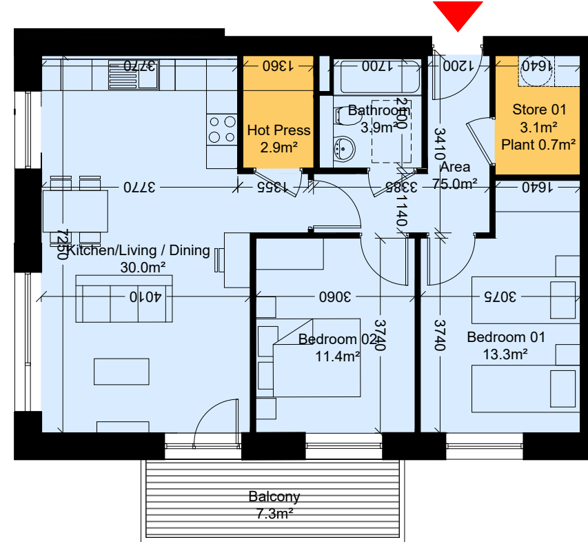
Unit Type J-06 Scale 1: 200 @A3
