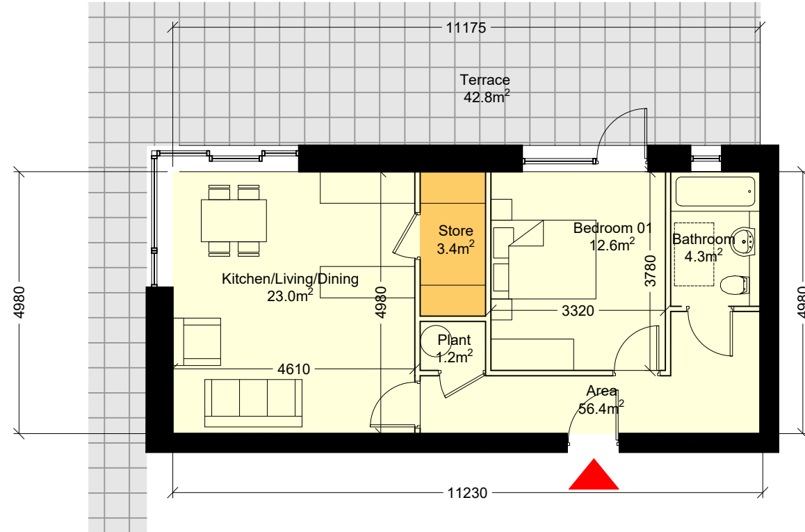
Unit Type J-03 Scale 1: 200 @A3
