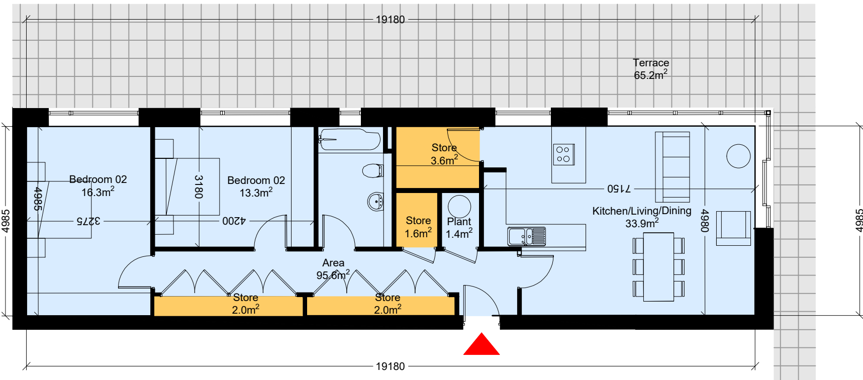
Unit Type J-04 Scale 1: 200 @A3
