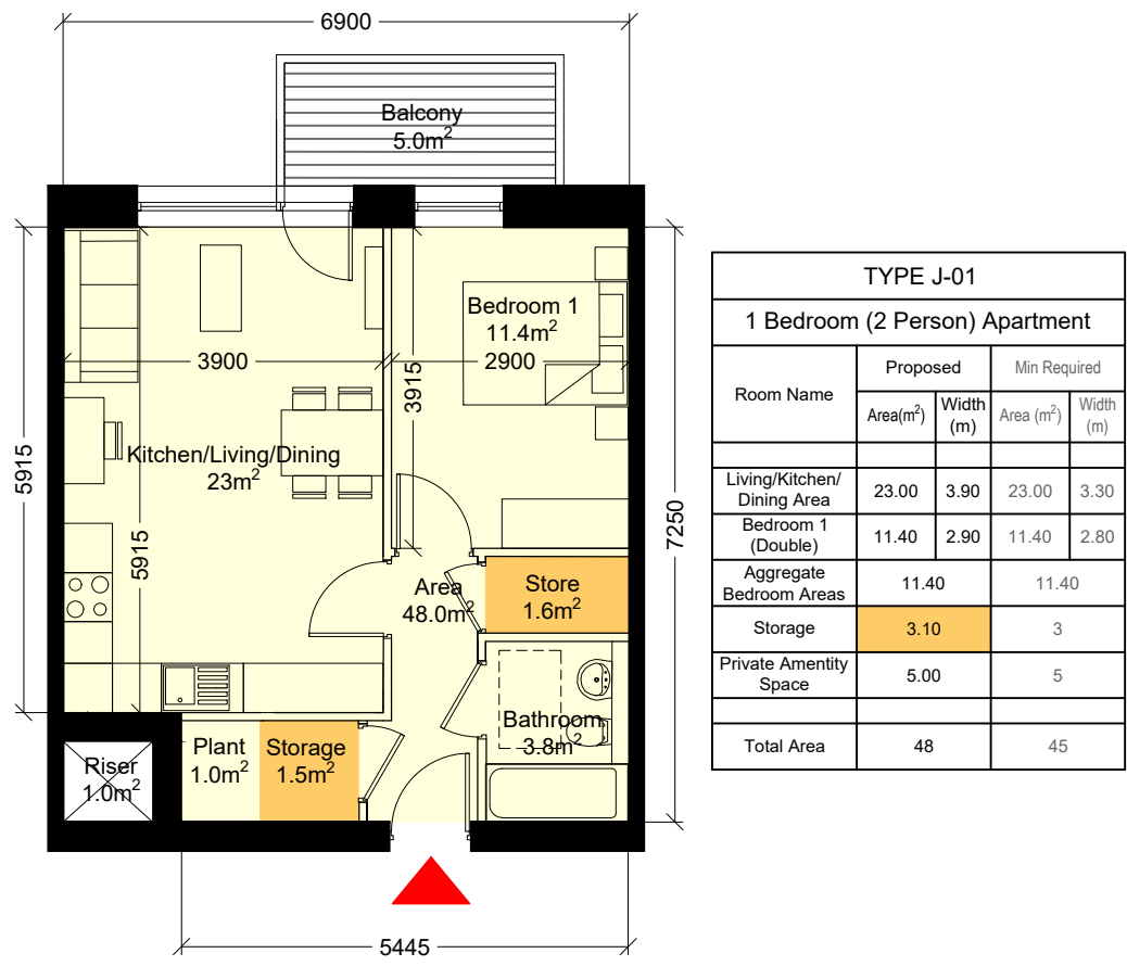
Unit Type J-01 Scale 1: 200 @A3
