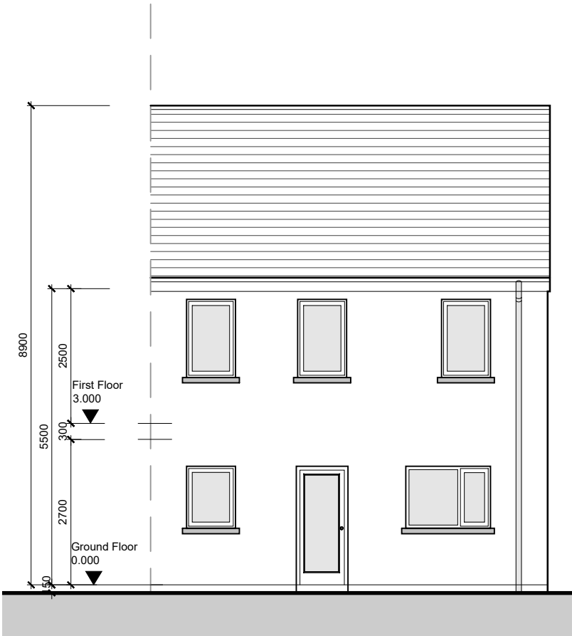
Rear Elevation
