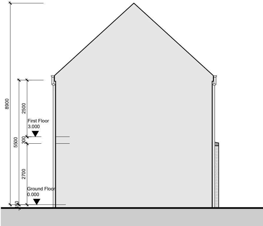
Side Elevation 01
