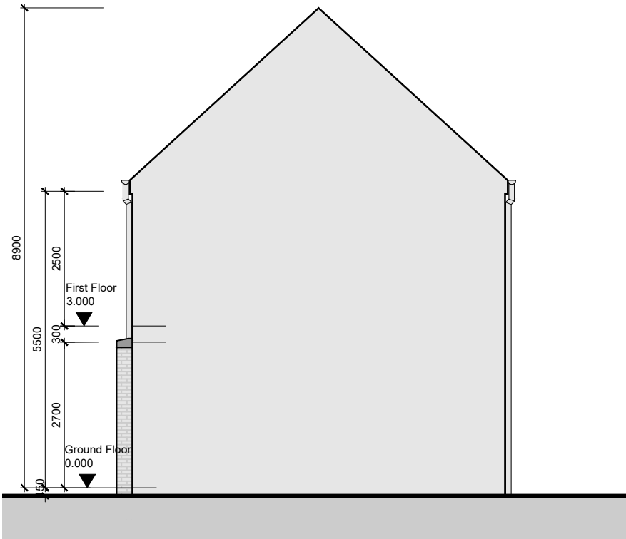
Side Elevation 02
