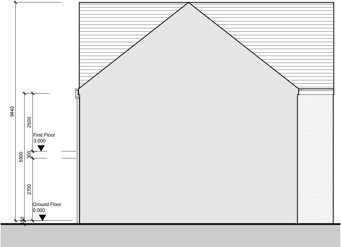
Side Elevation 02
