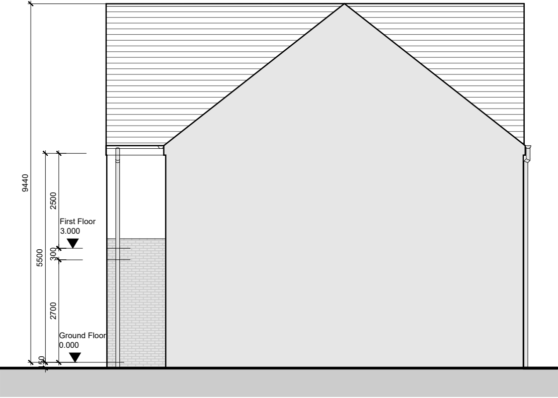
Side Elevation 02
