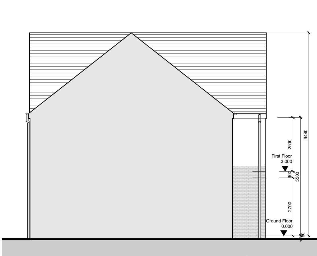
Side Elevation 02
