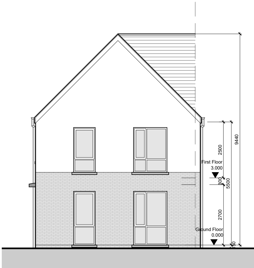
Side Elevation 01
