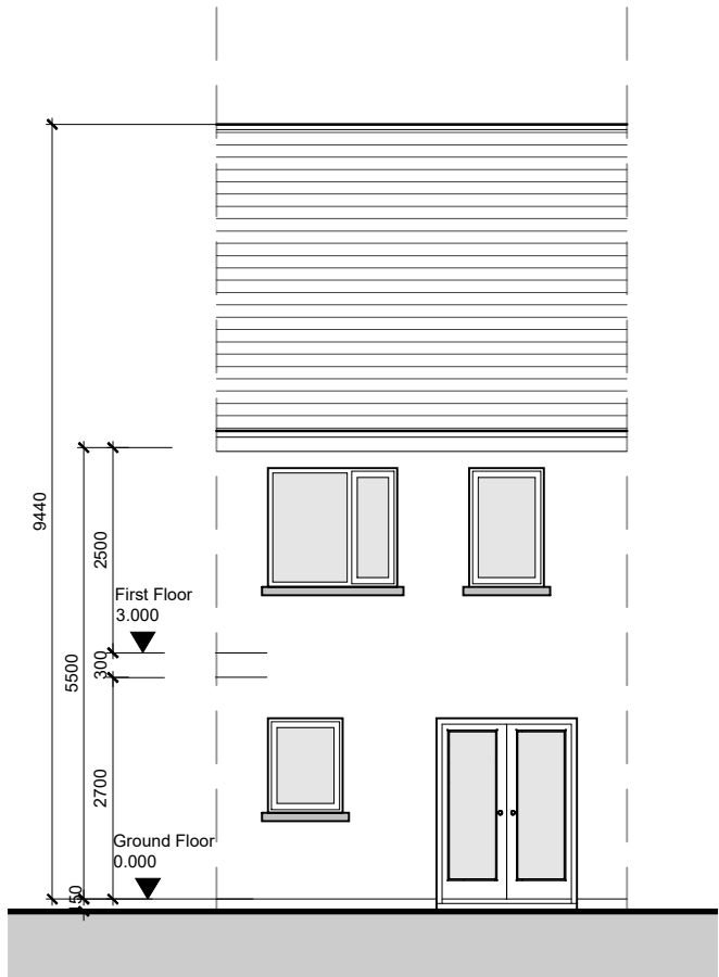
Rear Elevation
