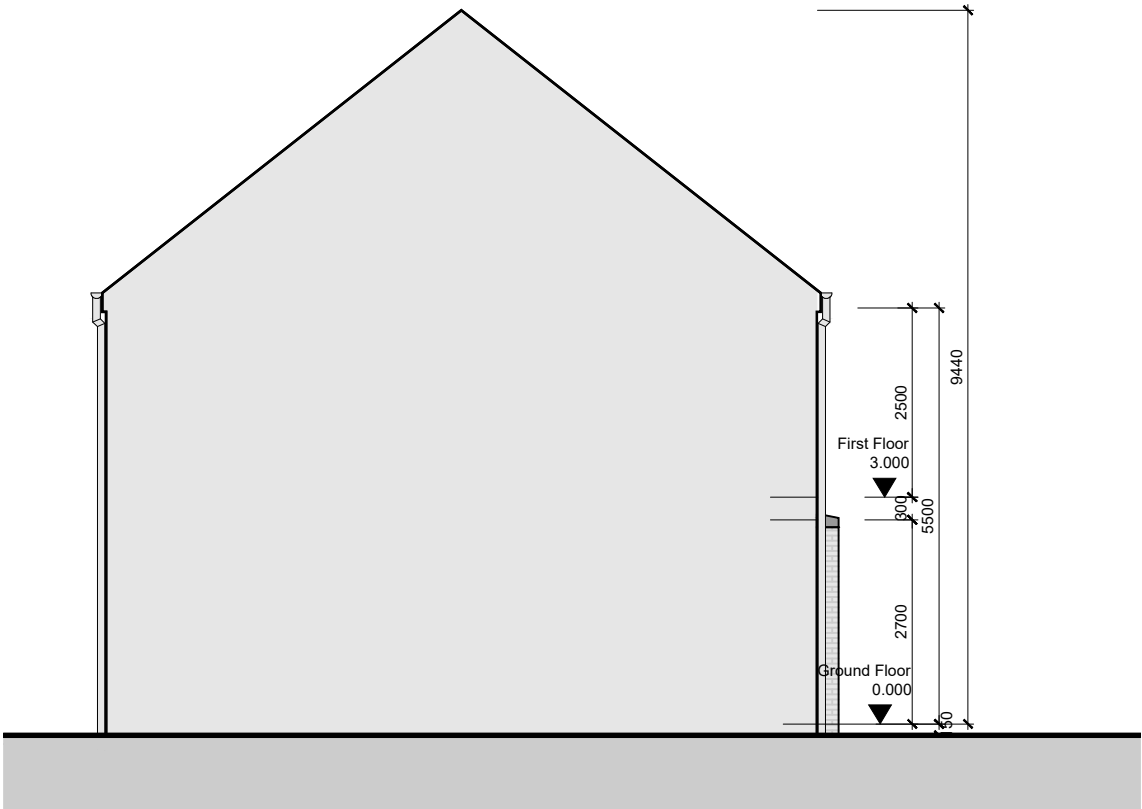
Side Elevation 02
