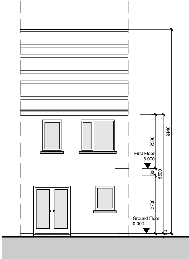
Rear Elevation
