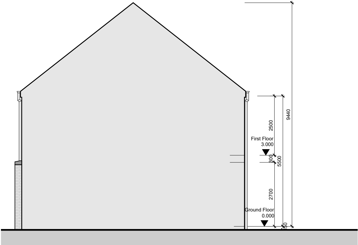
Side Elevation 01
