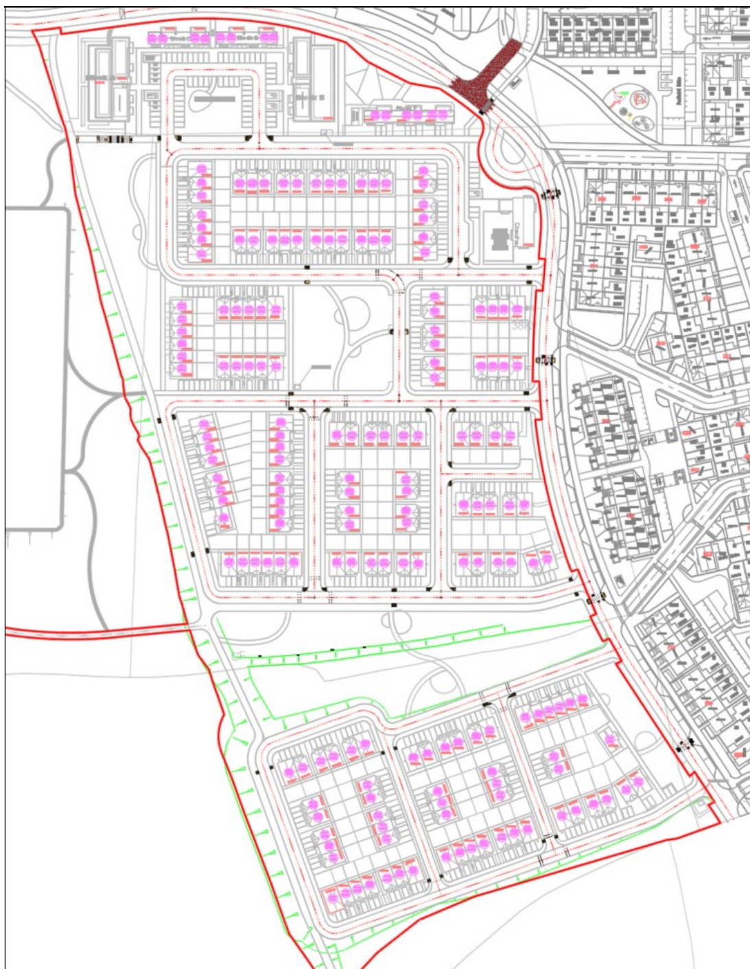
Figure 5.1: Overall proposed estate roads with earthwork lines
