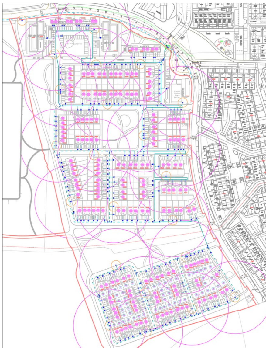
Figure 8.1: Overview of Watermain Network
