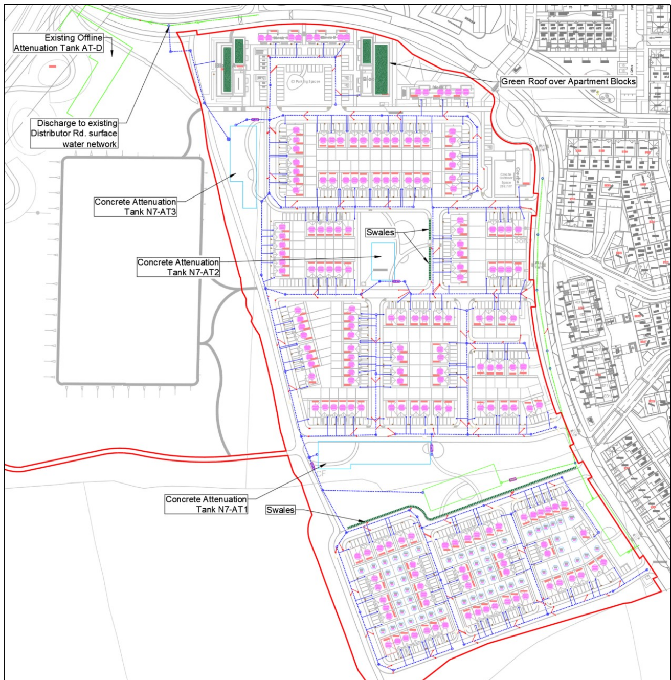
Figure 6.3: Overview of proposed storm network with attenuation tanks
